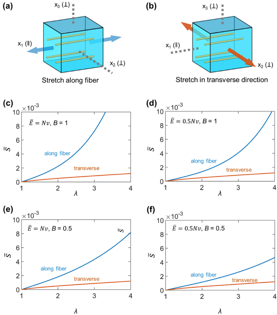
Fig. 4. Anisotropic stress response of \mu FRG with microfibers perfectly aligned in x_1 direction. Schematics of the \mu FRG under uniaxial tension (a) along the microfibrer direction and (b) in the transverse direction. Stress due to stretching the \mu FRG along the microfibrer direction (blue lines) and stretching along the transverse direction (orange lines) are plotted with various fiber properties: (c) \bar{E} = N\nu , B = 1 , (d) \bar{E} = 0.5N\nu , B = 1 , (e) \bar{E} = N\nu , B = 0.5 , and (f) \bar{E} = 0.5N\nu , B = 0.5 .
